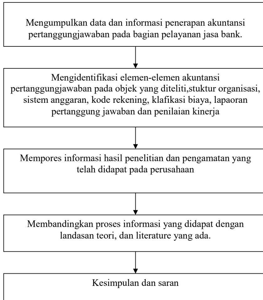
Gambar 3.1 Model Analisis
