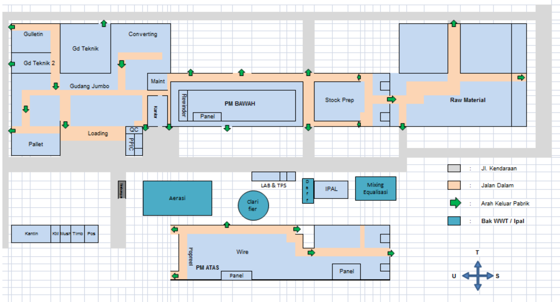
DENAH PT. STAR PAPER SUPPLY
