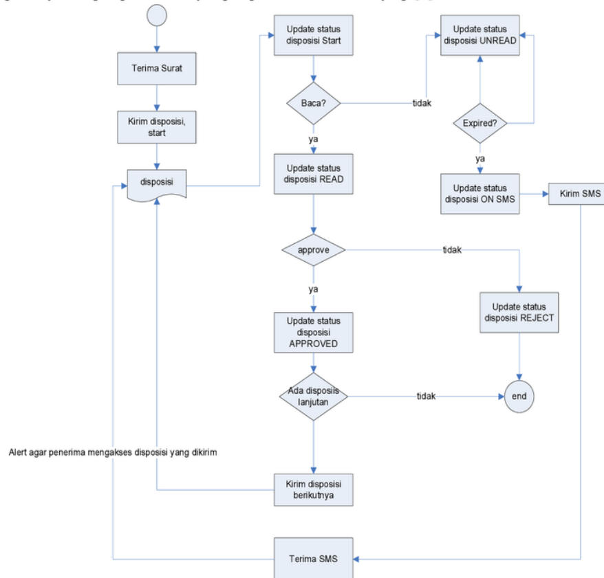
Gambar 1. Workflow Disposisi Online
