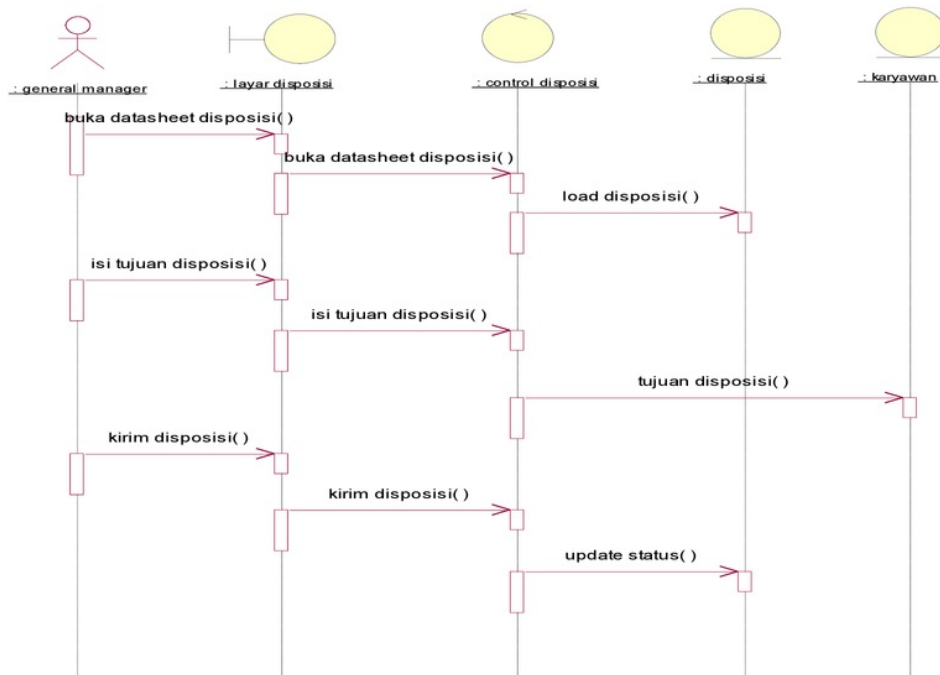
Gambar 4. Sequence Pengiriman Disposisi
