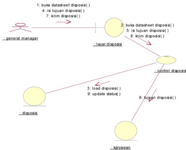
Gambar 6. Collaboration Diagram Disposisi
