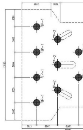
Denah Group Tiang
