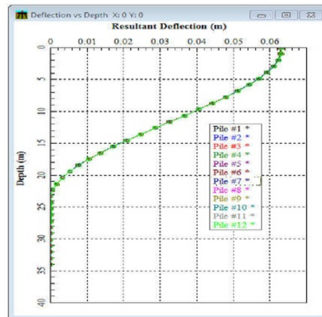
Alternatif 1 (Fy = 1200 kN) Deformasi Lateral: 6.3 cm
