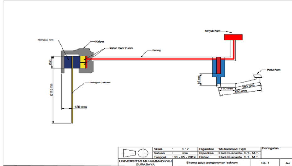
Gambar 2. 9 Distribusi gaya pengereman cakram (sumber : penelitian (2019))
