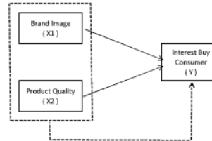
Figure 1 Conceptual Framework
