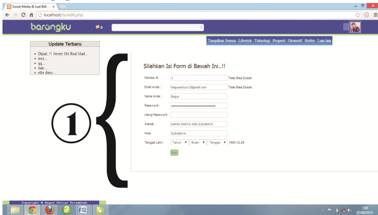
Gambar 4.6 : Halaman Edit.php
