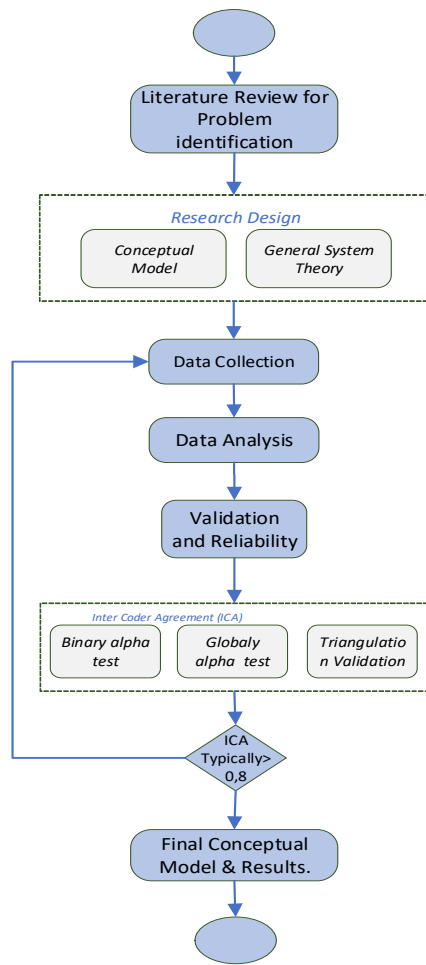
Fig. 1. Research Stages
