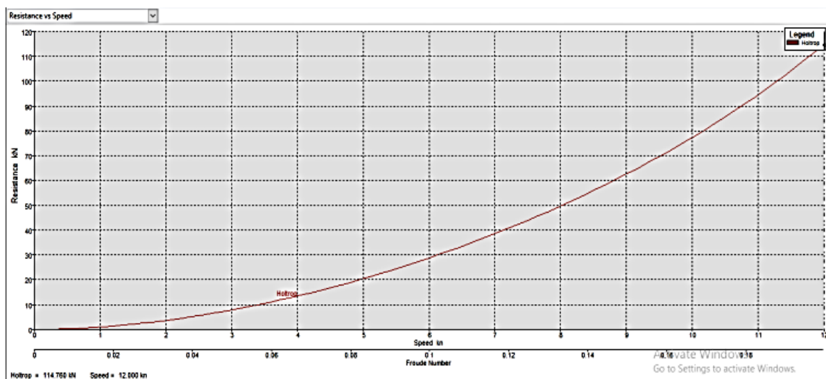
Figure 4 Graph of Resistance - Ship Speed
