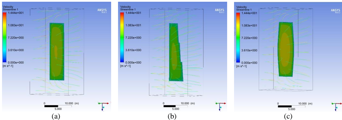
Figure 11 Simulation with wind direction angle 30^\circ M 1 (a), M 2 (b), M 3 (c)
