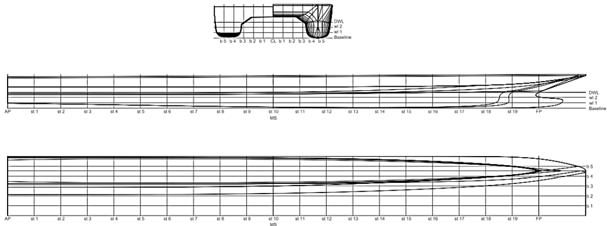
Figure 3 Lines Plan Catamaran
