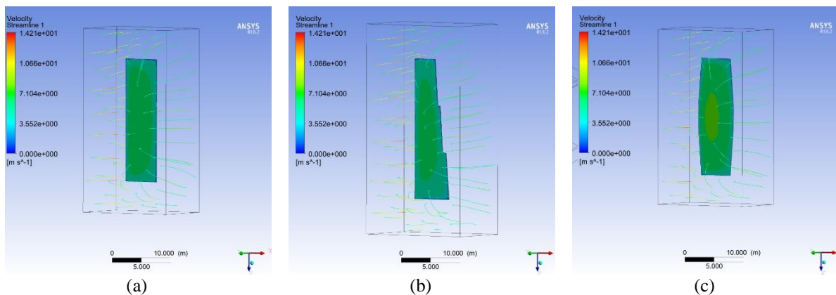
Figure 12 Simulation with wind direction angle 45^\circ M 1 (a), M 2 (b), M 3 (c)
