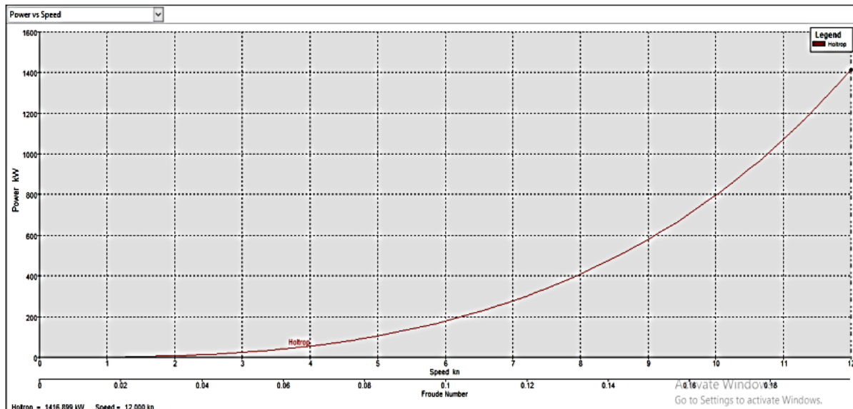
Figure 5 Graph of Ship Power - Ship Speed
