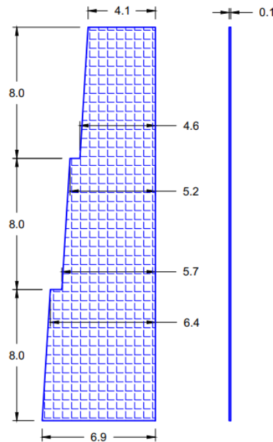
Figure 8 Model M_2
