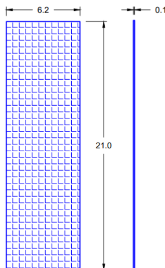
Figure 7 Model M_1
