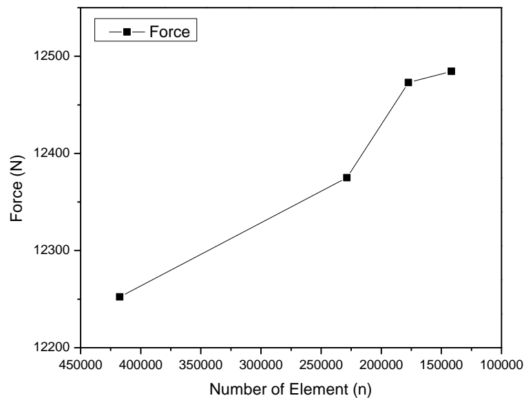
Figure 2 Grid Independence Study
