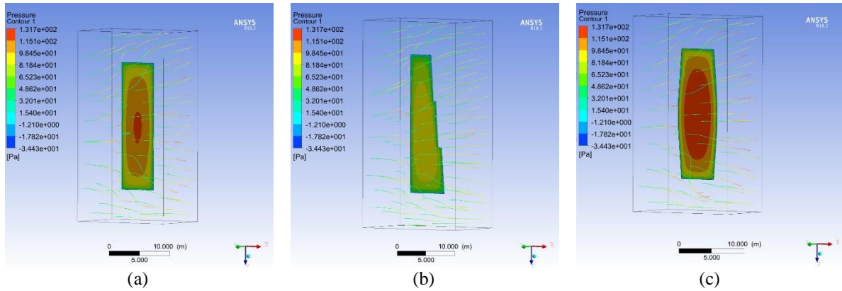
Figure 10 Simulation with wind direction angle 0^\circ M 1 (a), M 2 (b), M 3 (c)
