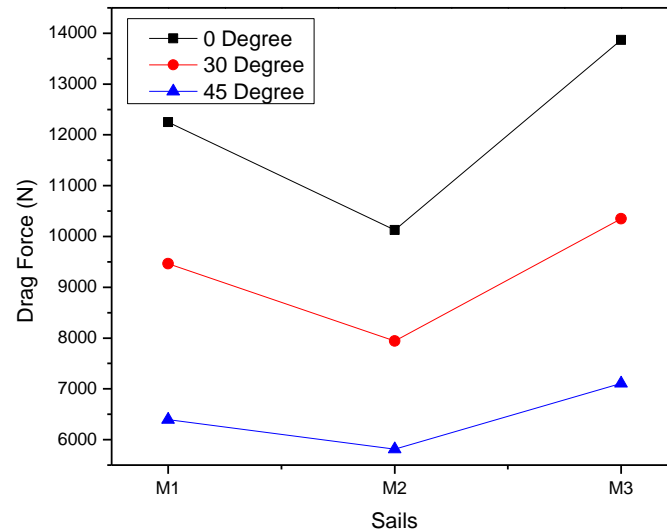
Figure 13 Simulation Result on various angle
