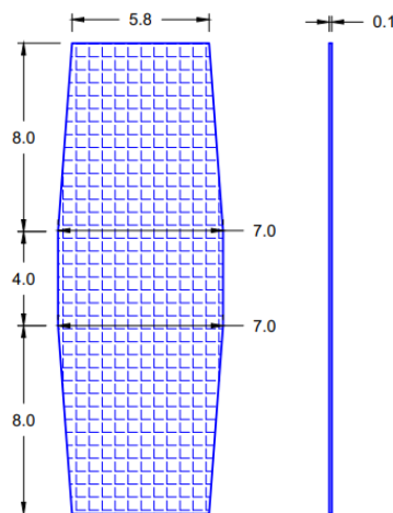
Figure 9 Model M_3
