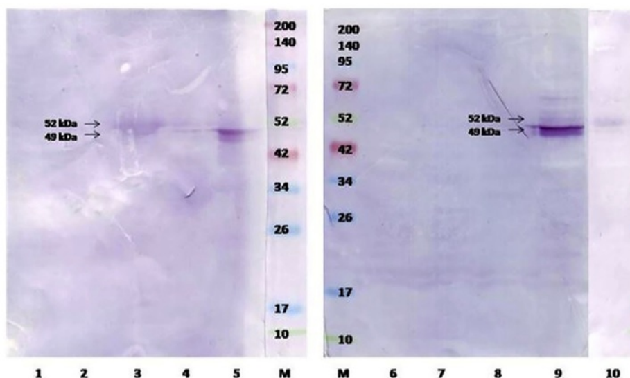
Figure 1. The results of western blot of bacterial sample OMP. Lane 1: OMP Streptococcus α-haemolyticus M1, lane 2: OMP E. coli M4, lane 3: OMP S. aureus M10, lane 4: OMP S. epidermidis M18 and lane 5: OMP S. aureus M19, which blotted with s-IgA cervix uteri M10, respectively. Lane 6: OMP E. coli M4, lane 7: OMP Streptococcus α-haemolyticus M11, lane 8: OMP S. epidermidis M18, lane 9: OMP S. aureus M19 and lane 10: OMP S. aureus M10, which blotted with s-IgA cervix uteri M19. M: marker.
