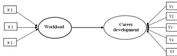
Fig 1. Conceptual Framework
