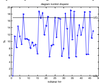
Gambar 4. Plot Diagram Kontrol Dispersi Data Agustus 2007 (Fase II)
