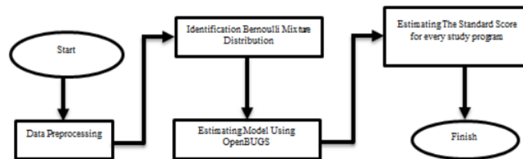
Figure 1. Research Design for Modelling Bernoulli Mixture Model.
