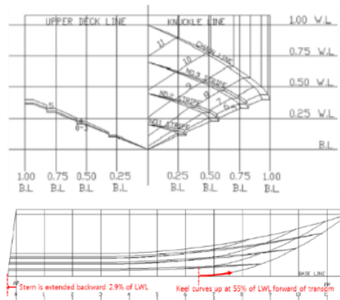
Gambar 1. Geometri 2-D VPS
