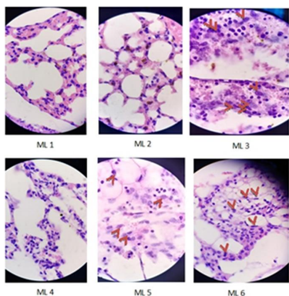
Fig. 2. Histology of lungs M. musculus in treatment Lactobacillus acidophilus , microscopic observation with 100× magnification of objective lens.
