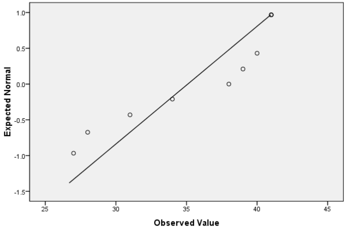
Normal Q-Q Plot of AUTORITATIF
