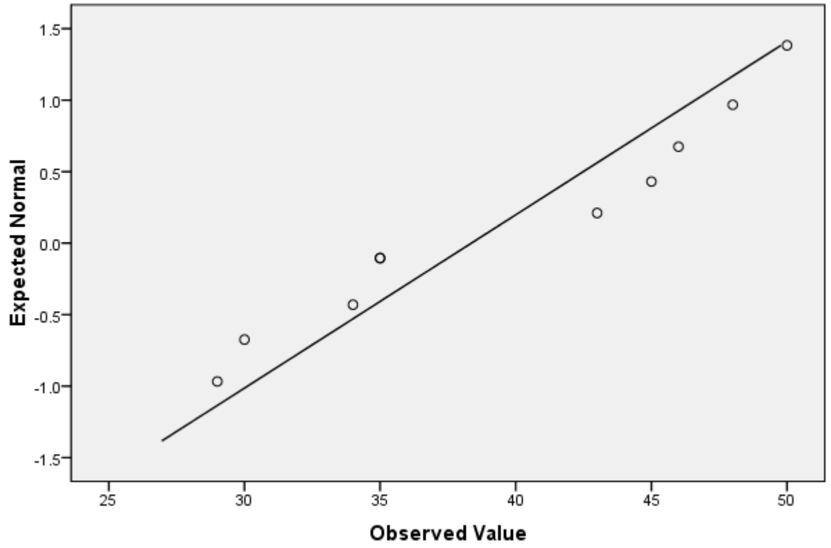
Normal Q-Q Plot of OTORITER
