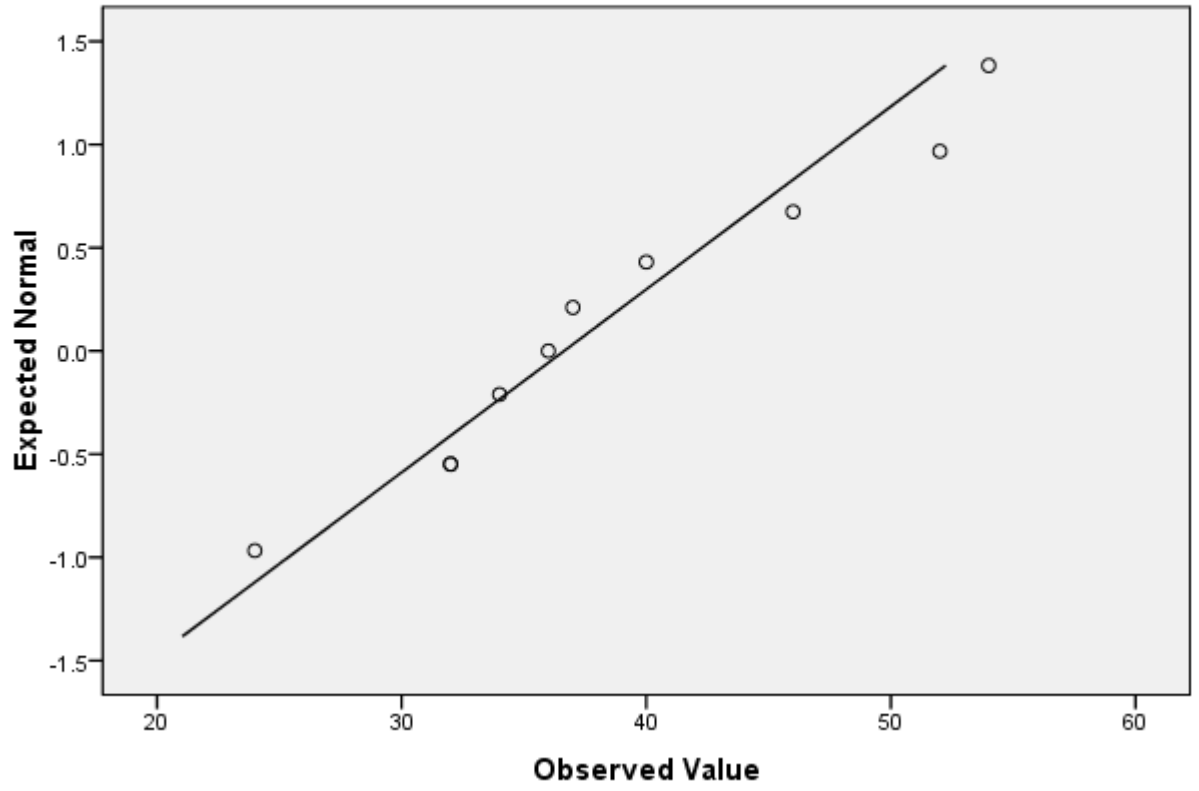
Normal Q-Q Plot of PERMISIF
