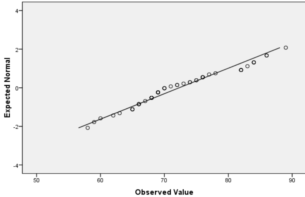
Normal Q-Q Plot of VAR00003
