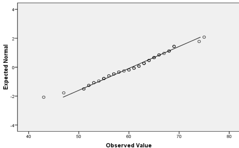
Normal Q-Q Plot of VAR00002
