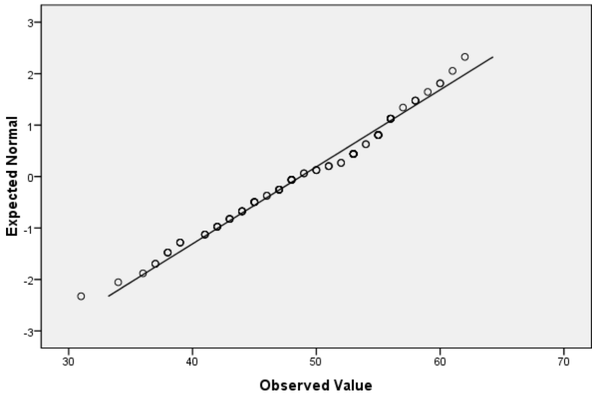
Normal Q-Q Plot of Fashion Involvement
