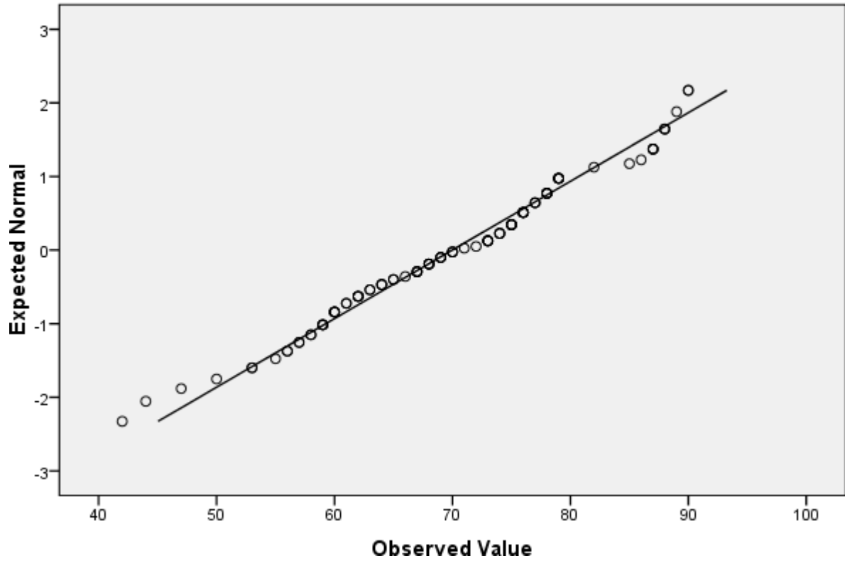
Normal Q-Q Plot of Hedonic Consumption Tendency
