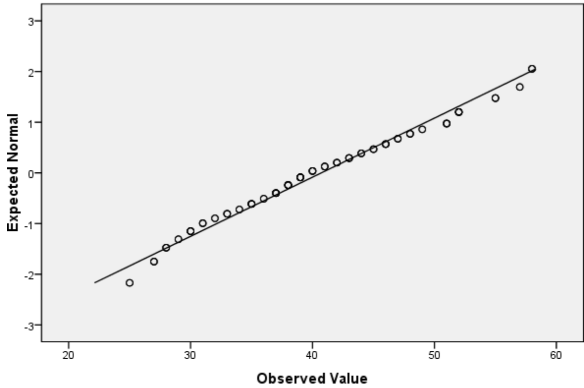
Normal Q-Q Plot of Impulsive Buying
