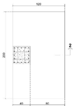
DET. DROP PANEL TYPE 2 SKALA 1 : 25
