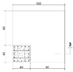
DET. DROP PANEL TYPE 3 SKALA 1 : 25
