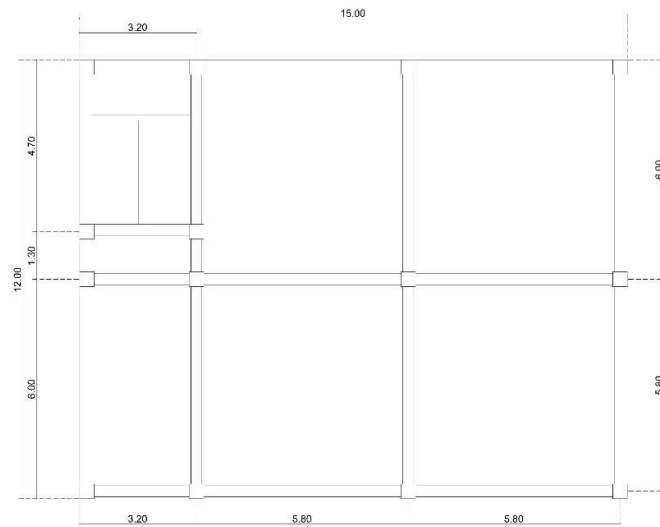
DENAH LANTAI 1 SKALA 1 : 100
