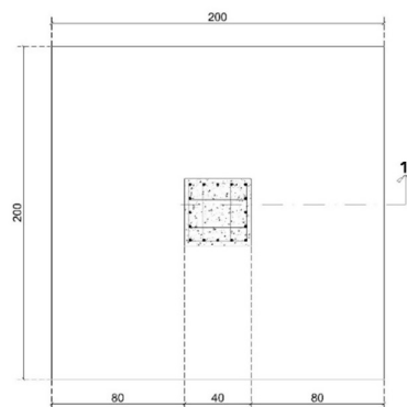
DET. DROP PANEL TYPE 1 SKALA 1:25
