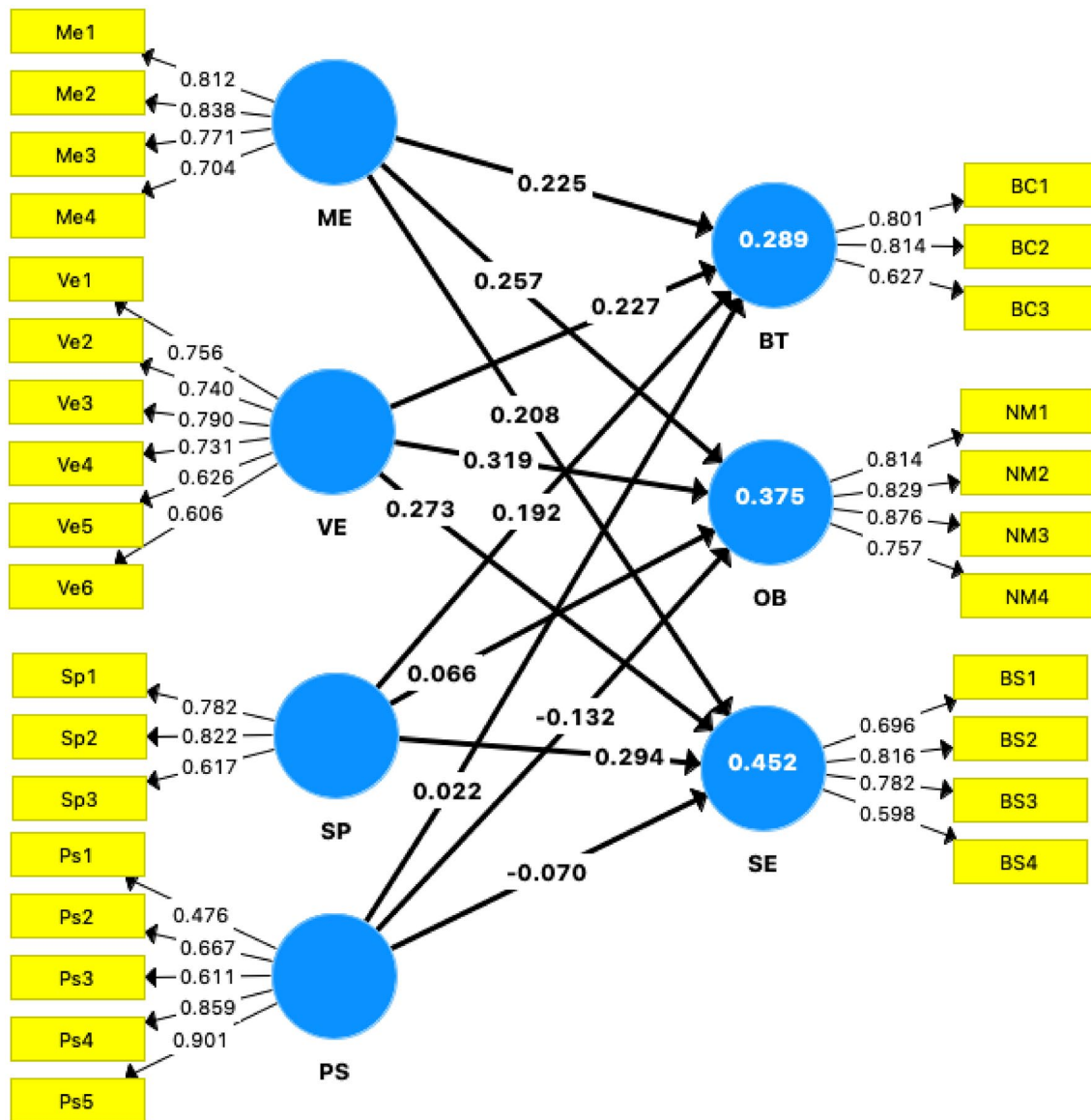
Fig. 1 The result of structural equation modeling evaluation. ME Mastery Experience, VE Vicarious Experience, SP Social Persuasion, PS Physiological State, OB Goal orientation beliefs, SE Self-efficacy, BT Beliefs about the role of mathematics teacher
