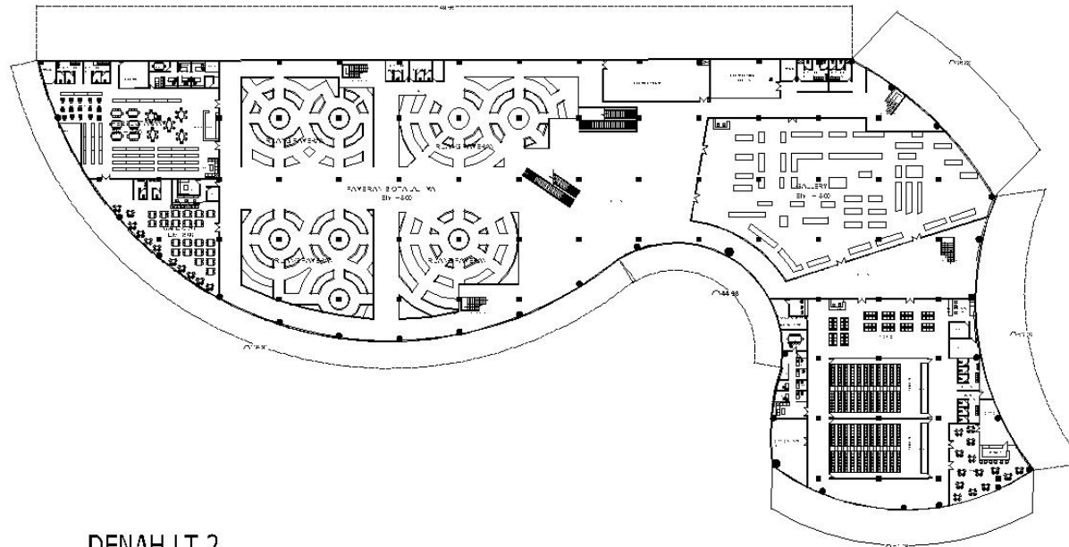
DENAH LT 2 MUSEUM BIOTA LAUT KENJERAN SKALA 1:500
