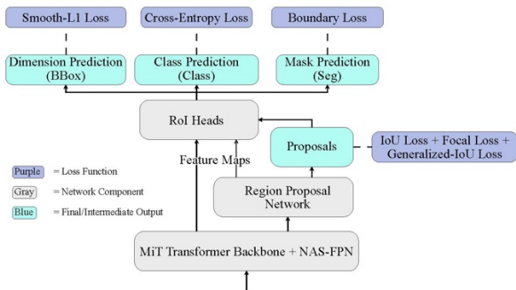
Figure 2. The loss functions utilized during training and their corresponding outputs.
