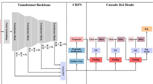
Figure 1. Our proposed network utilizes two-stage approach.
