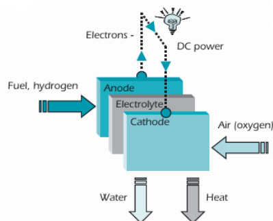
Gambar 6.1 Konsep fuel cell
