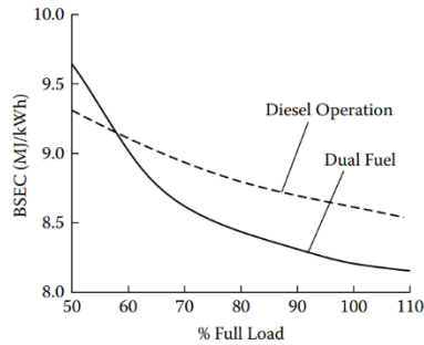
Gambar 5.1. Brake Spesific Energy Consumption (BSEC) DDF Vs Single (Danyluk, P.R., ASME, 1993).
