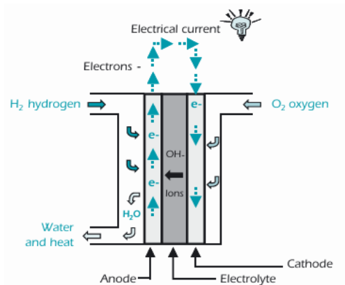
Gambar 6.5. Fuel cell jenis Alkaline
