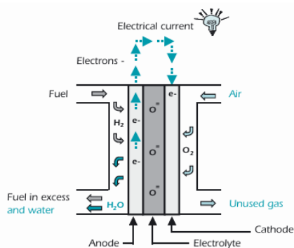
Gambar 6.3. Solid Oxide Fuel Cell
