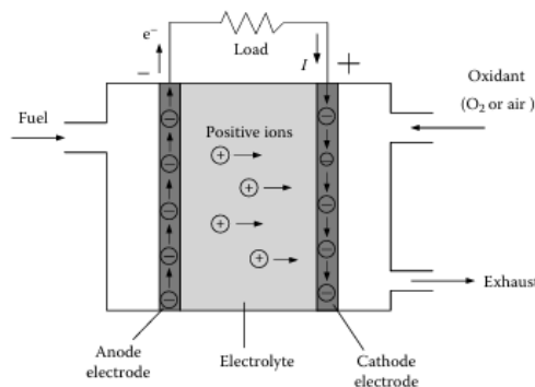
Gambar 6.6. Operasi dasar fuel cell
