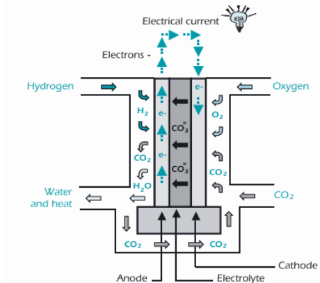
Gambar 6.4. Molten Carbonate Fuel Cell
