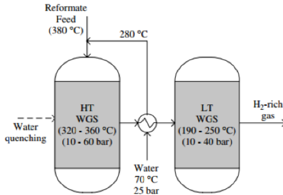
Gambar 2.4 Proses reaksi water gas shift
