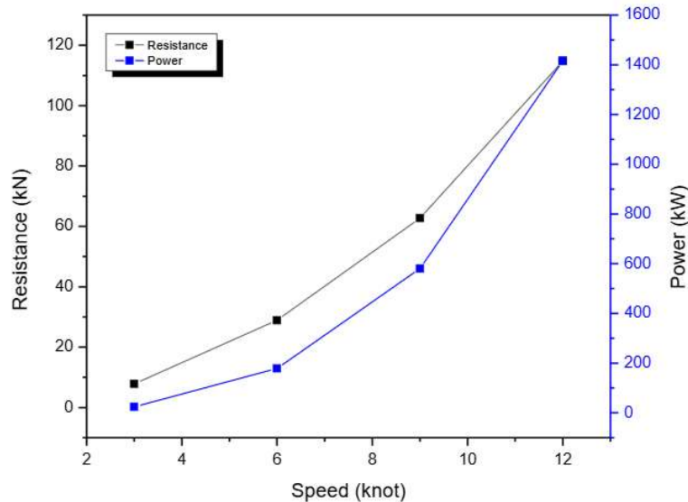
Figure 6. Ship Resistance – Ship Power Requirements
