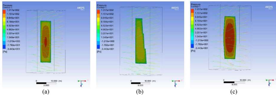
Figure 10. Simulation with Wind Direction Angle 0^\circ (a) M_1 , (b) M_2 , (c) M_3
