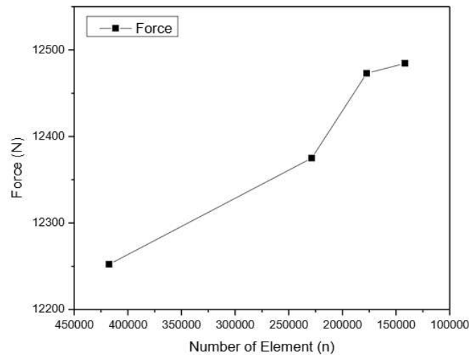
Figure 2. Grid Independence Study
