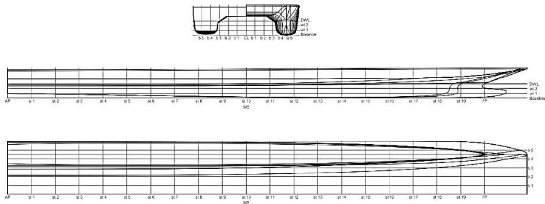
Figure 3. Lines Plan Catamaran
