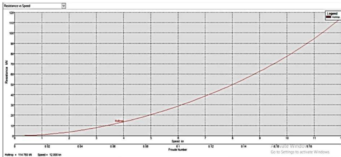
Figure 4. Graph of Resistance - Ship Speed
