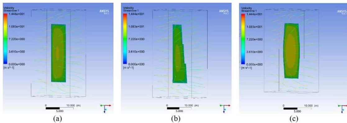
Figure 11. Simulation with Wind Direction Angle 30^\circ (a) M_1 , (b) M_2 , (c) M_3
