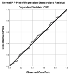
Figure 1. P-Plot Normality Test
