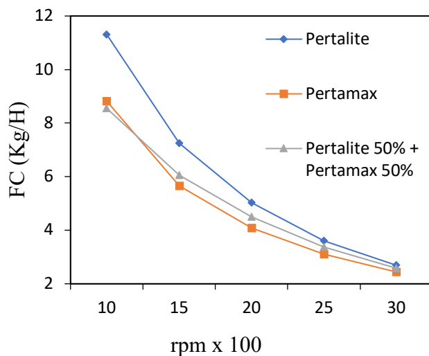
Gambar 4. Grafik Hubungan Putaran VS Fuel Consumption
