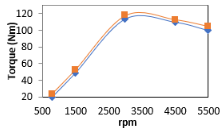
Figure 5. Torque of pertamax (♦) and pertamax turbo (■)
