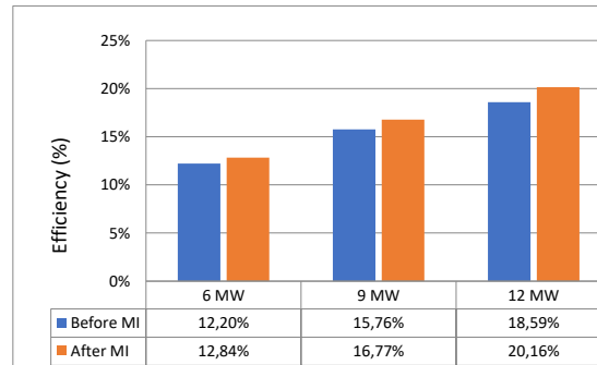
Figure 5. Cycle efficiency comparison of CTG 101
