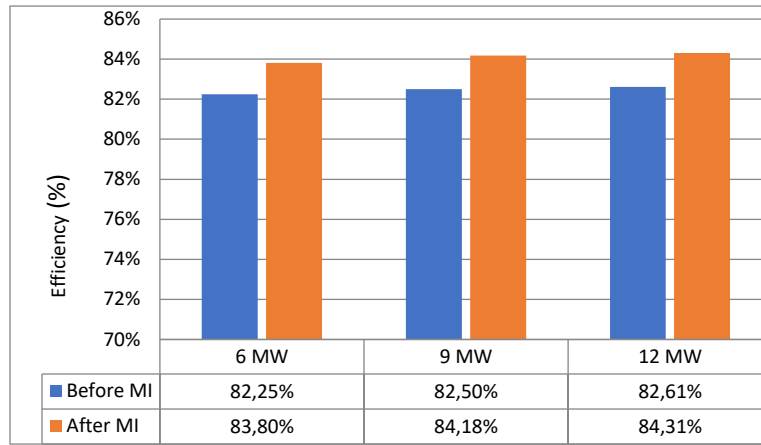
Figure 3. Compressor Efficiency Comparison of CTG 101
