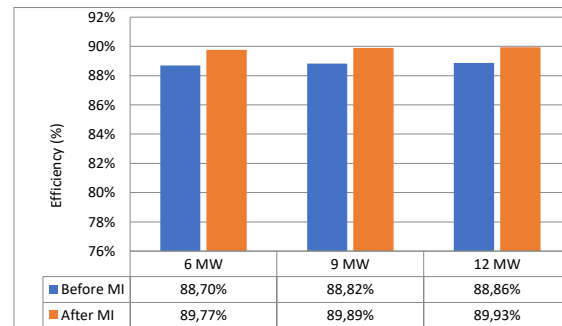
Figure 4. Turbine Efficiency Comparison of CTG 101
