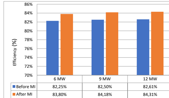
Figure 3. Compressor Efficiency Comparison of CTG 101
