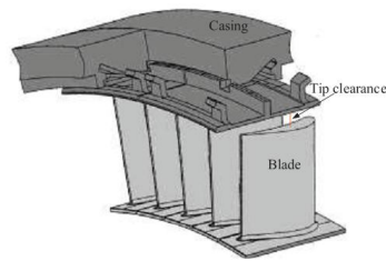
Figure 12. Blade Tip Clearance on Turbine
