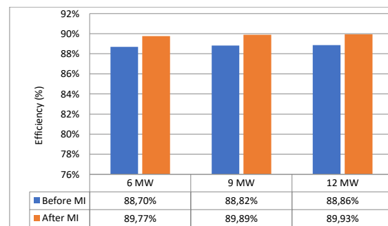
Figure 4. Turbine Efficiency Comparison of CTG 101
