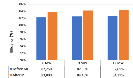
Figure 3. Compressor Efficiency Comparison of CTG 101
