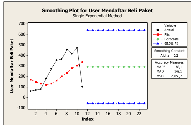
Gambar 5. Peramalan Smoothing Plot
