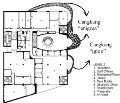
Gambar 5. Denah Lantai 2 Salvador Dali Museum Sumber : https://www.archdaily.com
