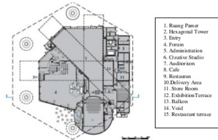
Gambar 10. Denah Lantai 1 Pompidou Centre Metz Sumber : https://aasarchitecture.com
