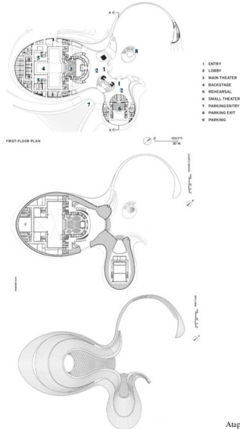
Gambar 21. Denah Lt 1, 2, dan Atap Harbin Opera House Sumber : https://www.archdaily.com
