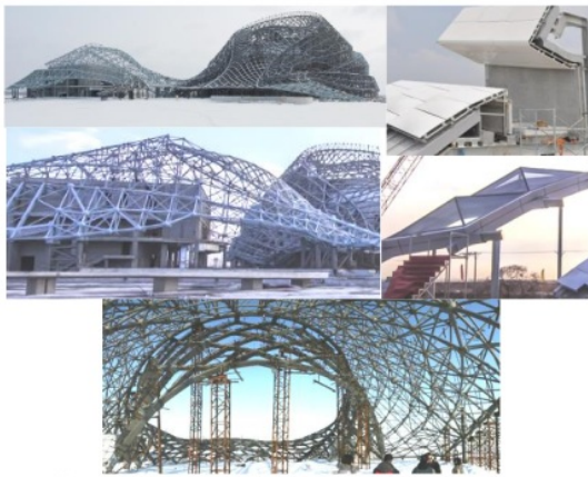
Gambar 22. Konstruksi Atap Harbin Opera House Sumber : https://www.archdaily.com
