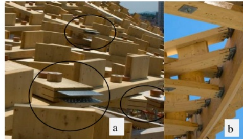
Gambar 15. Penumpu Atap Pompidou Centre Metz Sumber: https://www.centrepompidou-metz.fr
