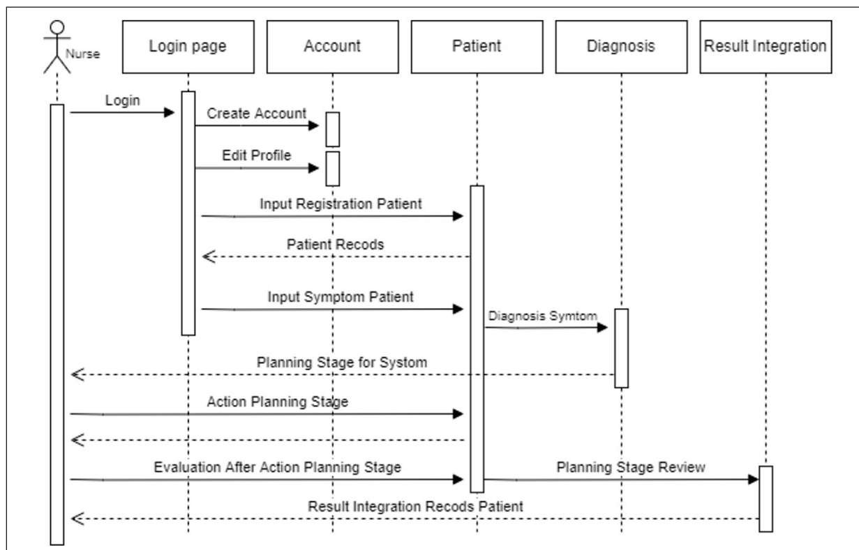
Figure 2. Sequence diagram MNCIPIS.
