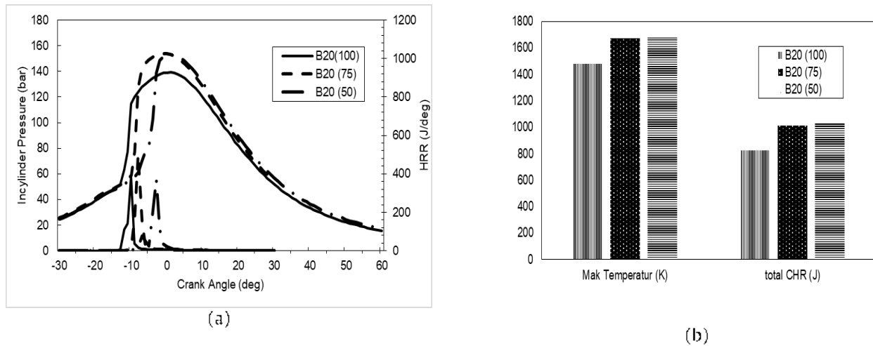
Figure 3. Graph of combustion incylinder pressure, HRR (a) and Max temperature, CHR (b) in variation of percentage of biodiesel – biogas
