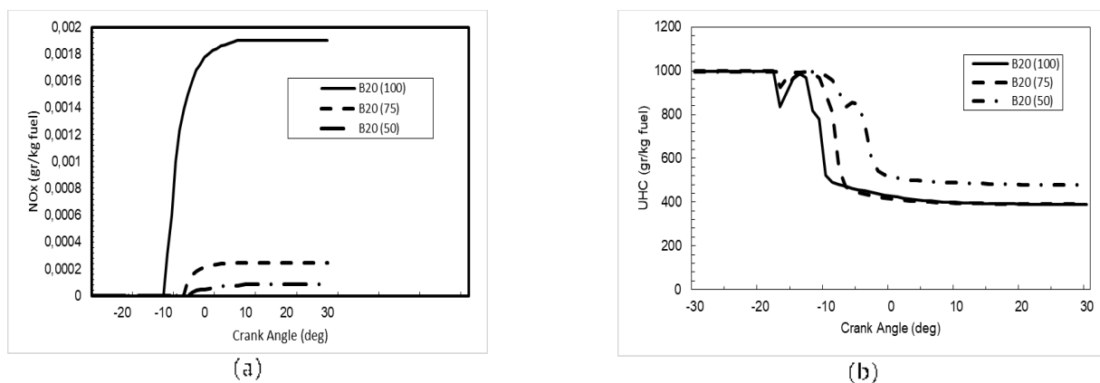
Figure 4. Graph of Emission NOx (a) and UHC (b) in variation percentage of biodiesel – biogas
