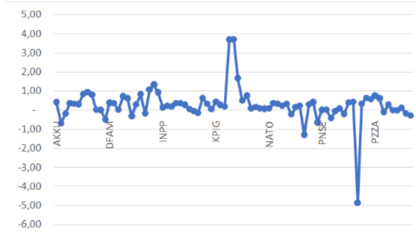
Graph 4. Grover's Analysis (G-Score)
