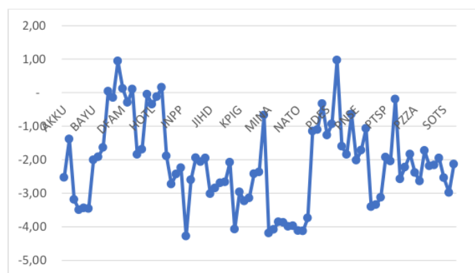
Graph 4. Zmijewski Analysis (X-Score)
