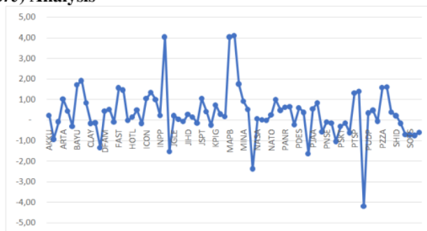
Graph 3. Springate Analysis (S-Score)
