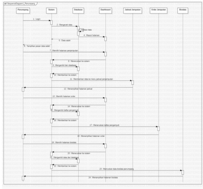
Gambar 4. Sequence Diagram Penumpang
