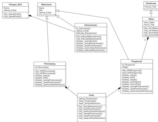
Gambar 5. Class Diagram BEPO
