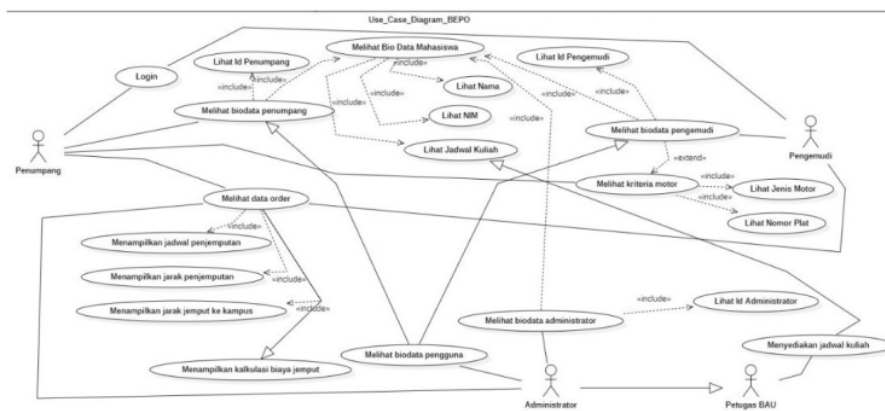
Gambar 3. Use Case Diagram BEPO
